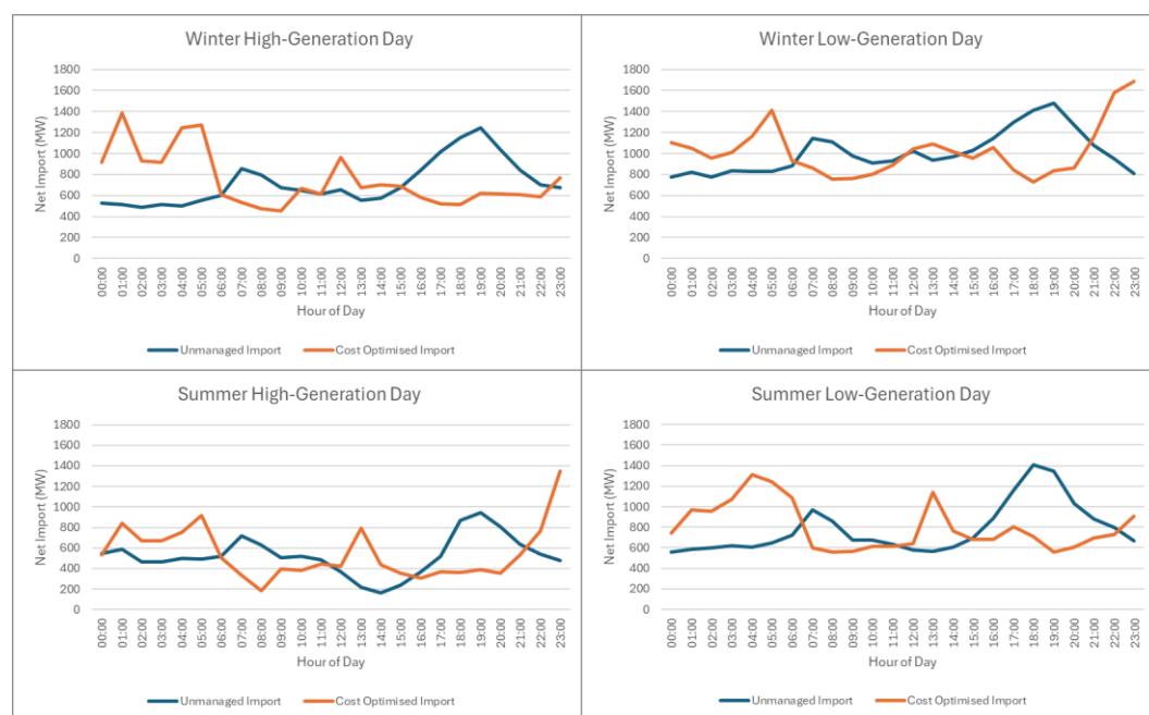
Figure 41 Impact on national demand profile in 2030 for Cost Optimised charging
