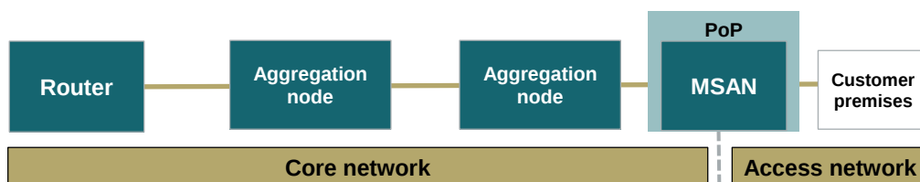
Figure 19. FTTC
